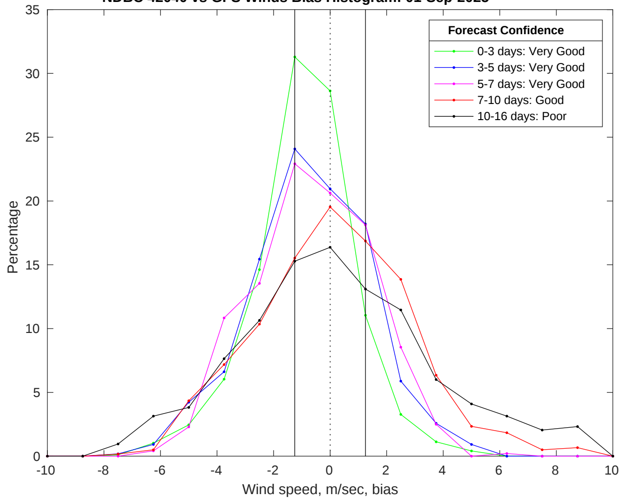
NDBC 42040 vs GFS Winds Bias Histogram: 01-Sep-2025
