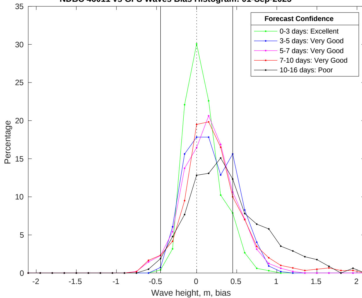
NDBC 46011 vs GFS Waves Bias Histogram: 01-Sep-2025
