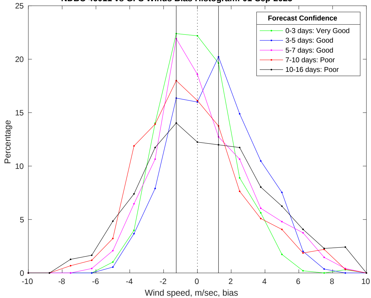
NDBC 46011 vs GFS Winds Bias Histogram: 01-Sep-2025
