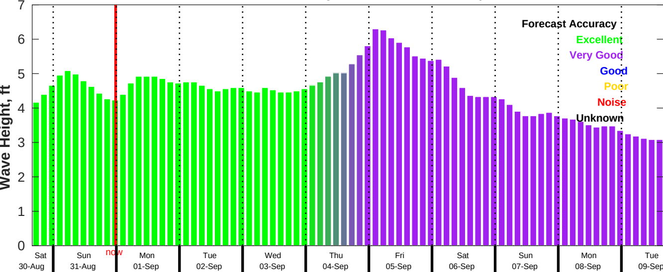
CMEMS Wave Forecast for NDBC 46011 from 30-Aug-2025 16:00:00 to 09-Sep-2025 16:00:00
