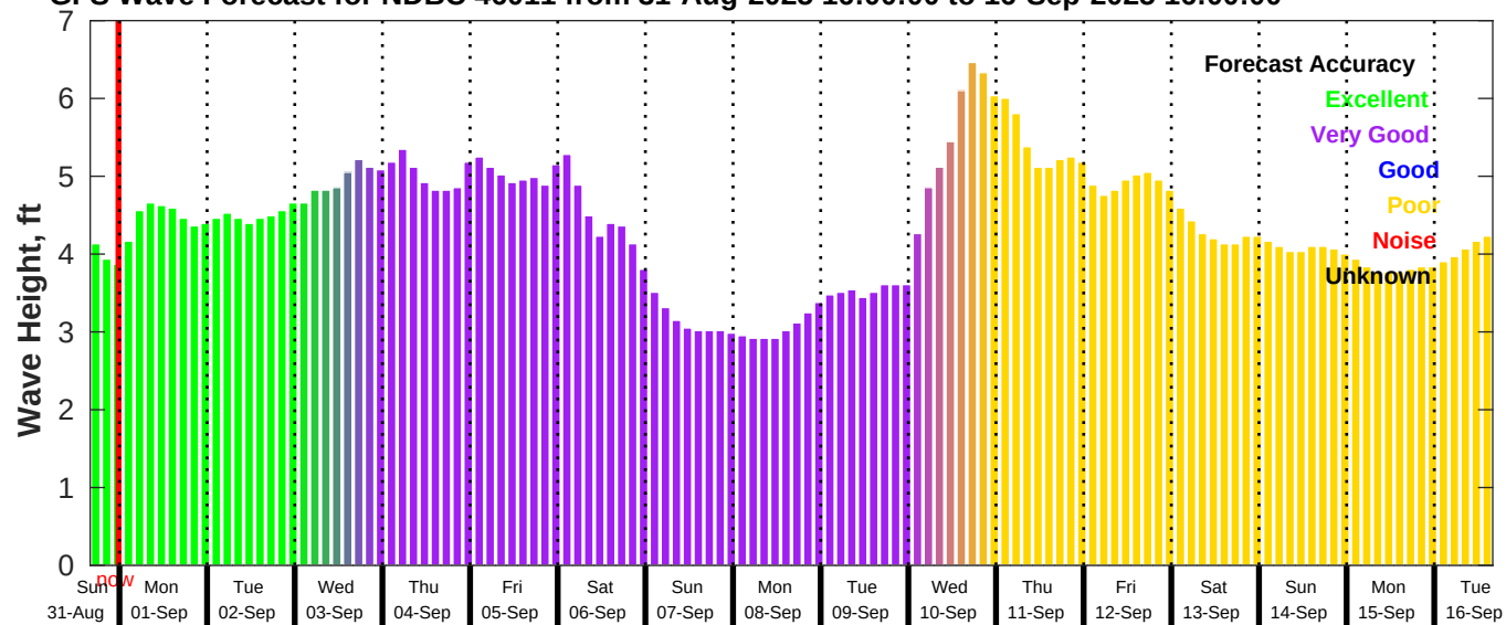
GFS Wave Forecast for NDBC 46011 from 31-Aug-2025 16:00:00 to 16-Sep-2025 16:00:00
