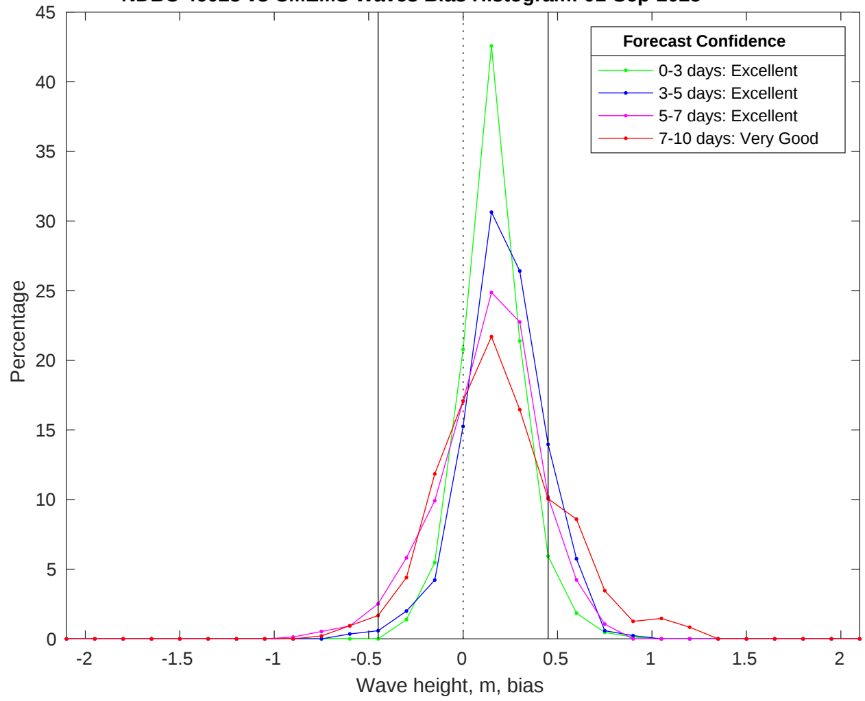
NDBC 46028 vs CMEMS Waves Bias Histogram: 01-Sep-2025
