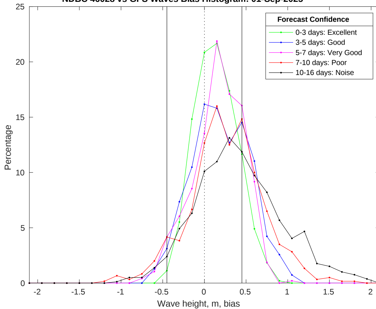
NDBC 46028 vs GFS Waves Bias Histogram: 01-Sep-2025
