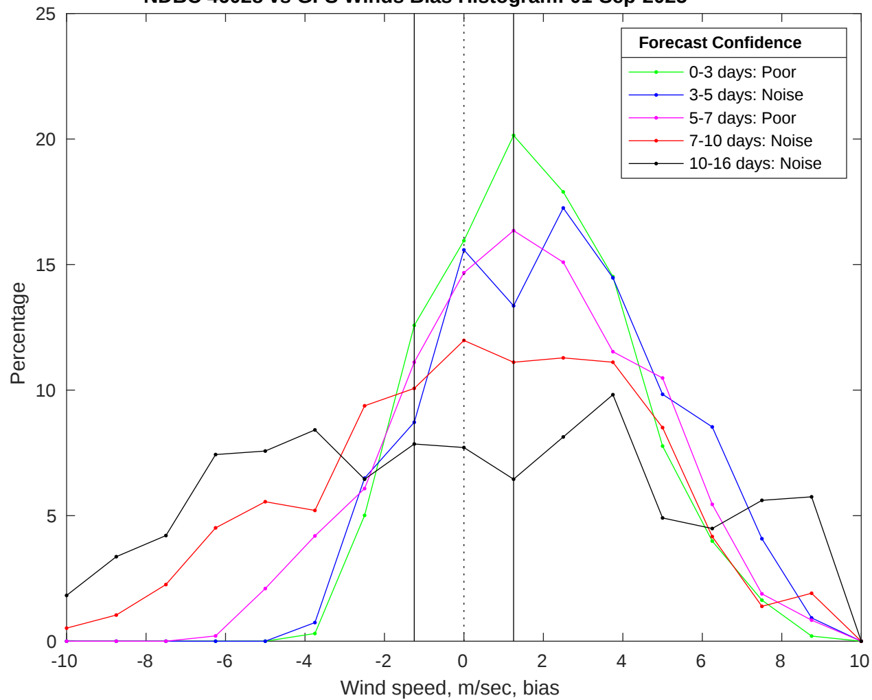
NDBC 46028 vs GFS Winds Bias Histogram: 01-Sep-2025
