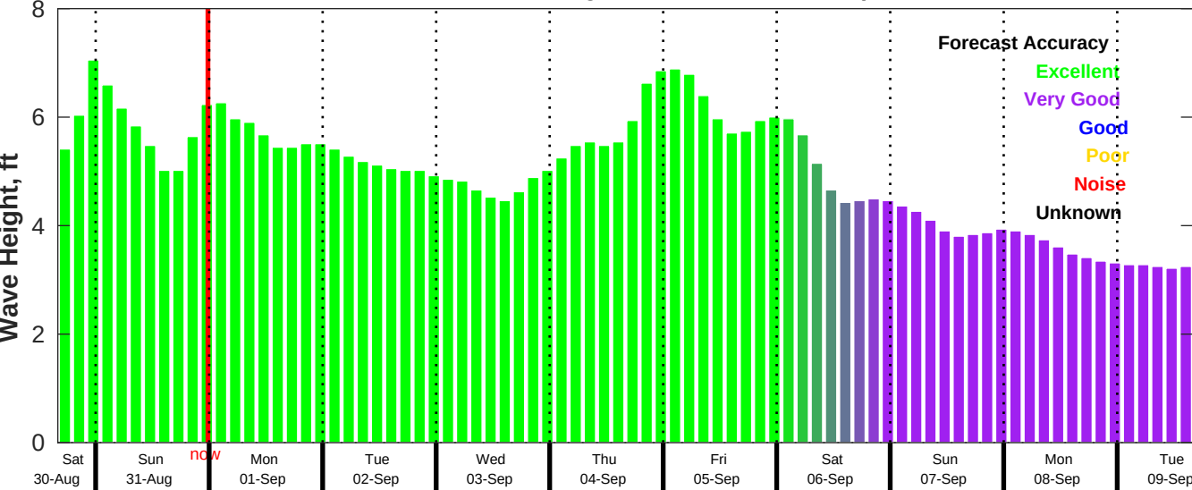
CMEMS Wave Forecast for NDBC 46028 from 30-Aug-2025 16:00:00 to 09-Sep-2025 16:00:00
