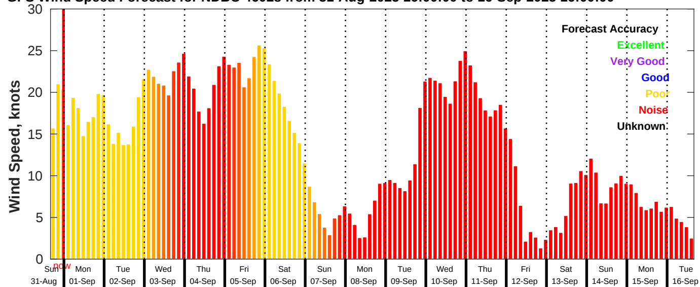
GFS Wind Speed Forecast for NDBC 46028 from 31-Aug-2025 16:00:00 to 16-Sep-2025 16:00:00
