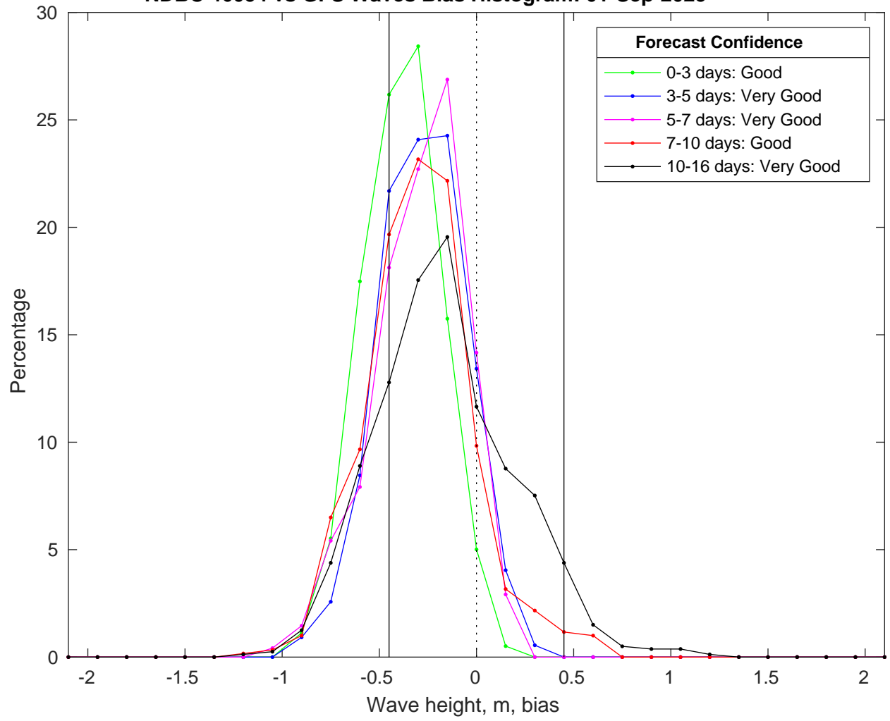
NDBC 46054 vs GFS Waves Bias Histogram: 01-Sep-2025
