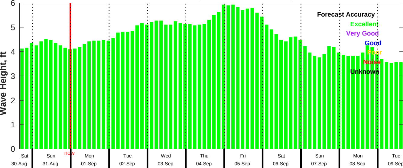
CMEMS Wave Forecast for NDBC 46054 from 30-Aug-2025 16:00:00 to 09-Sep-2025 16:00:00
