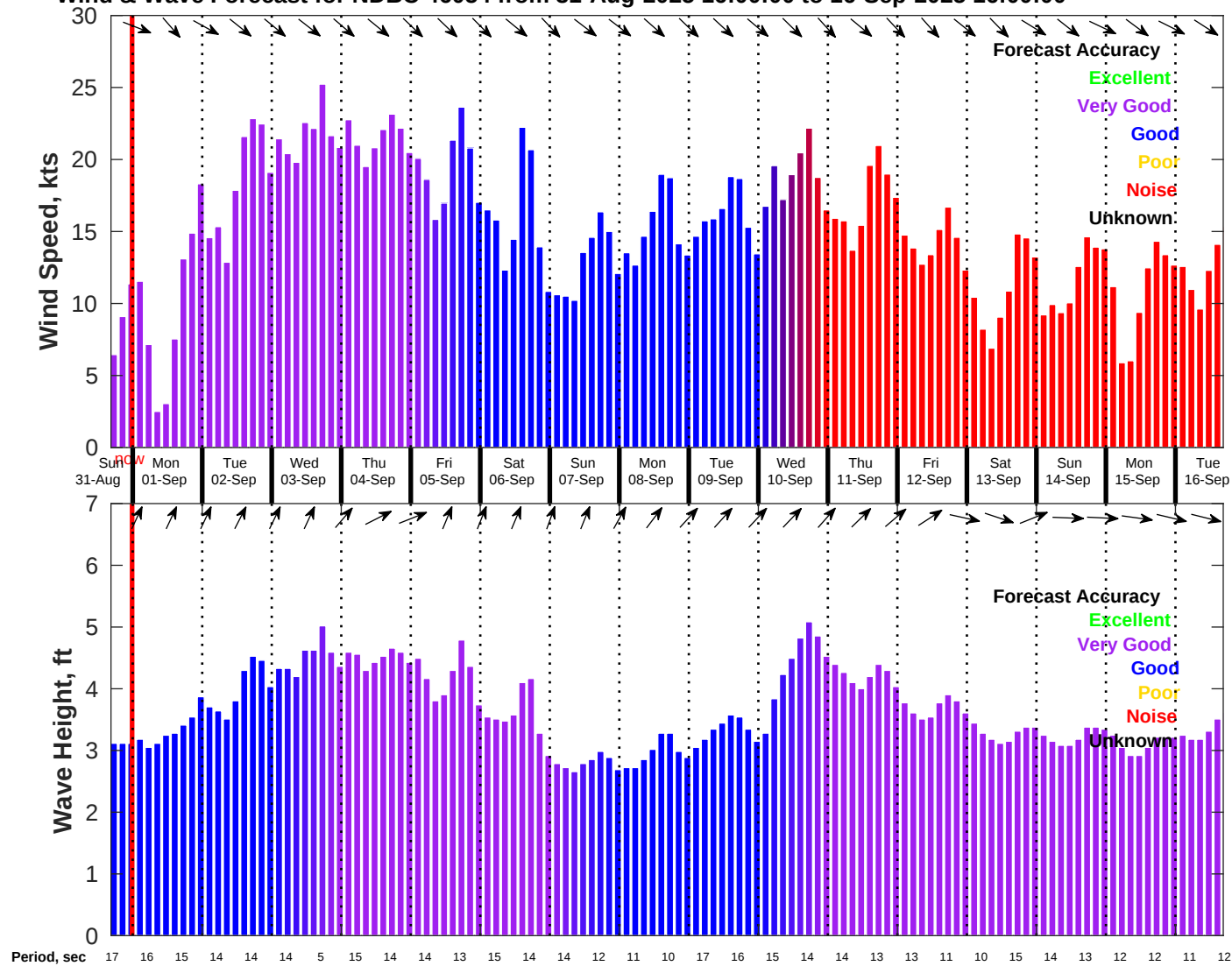
Wind & Wave Forecast for NDBC 46054 from 31-Aug-2025 16:00:00 to 16-Sep-2025 16:00:00
