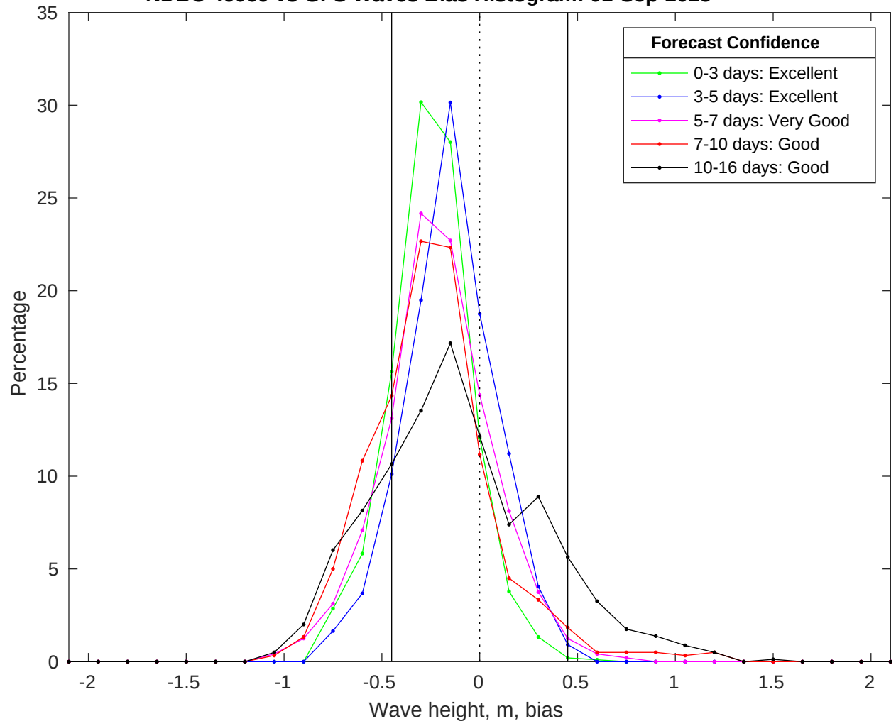
NDBC 46069 vs GFS Waves Bias Histogram: 01-Sep-2025
