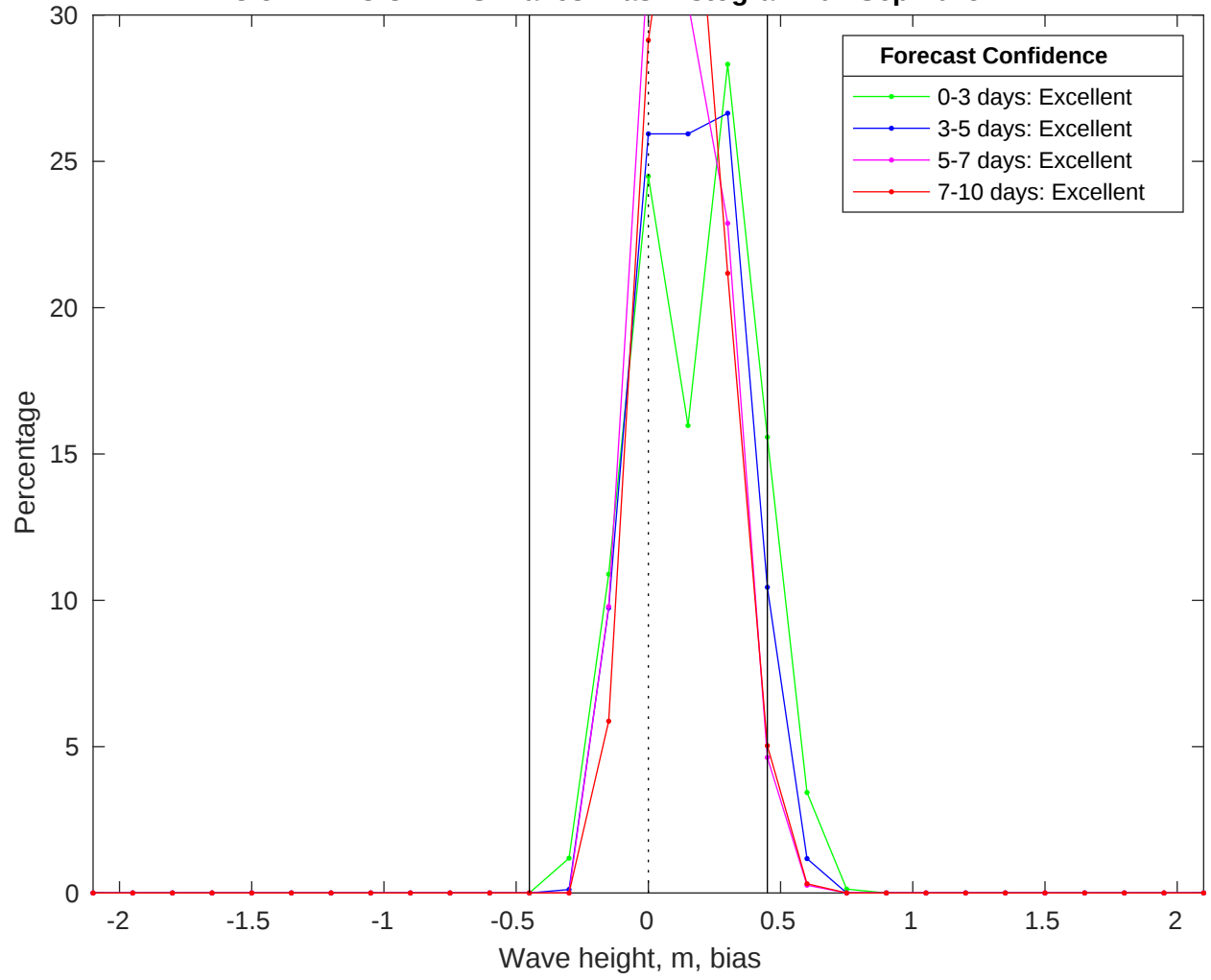
NDBC 51211 vs CMEMS Waves Bias Histogram: 01-Sep-2025
