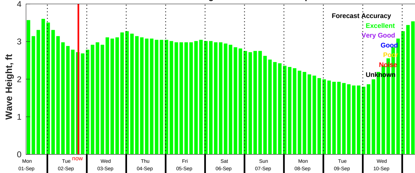
CMEMS Wave Forecast for NDBC 52211 from 31-Aug-2025 11:00:00 to 10-Sep-2025 11:00:00
