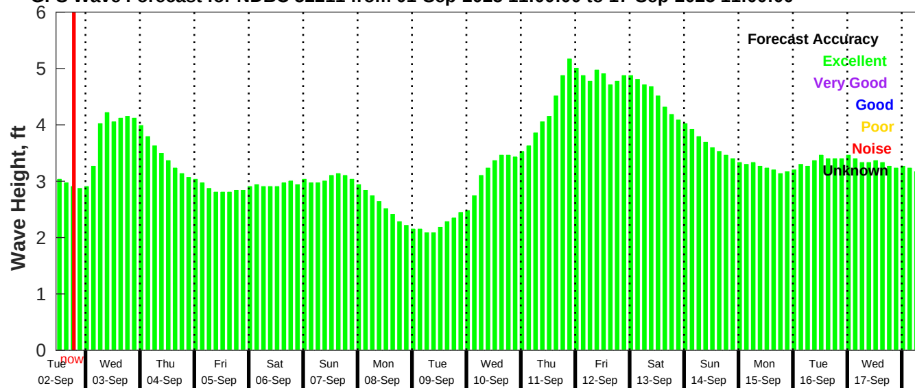
GFS Wave Forecast for NDBC 52211 from 01-Sep-2025 11:00:00 to 17-Sep-2025 11:00:00
