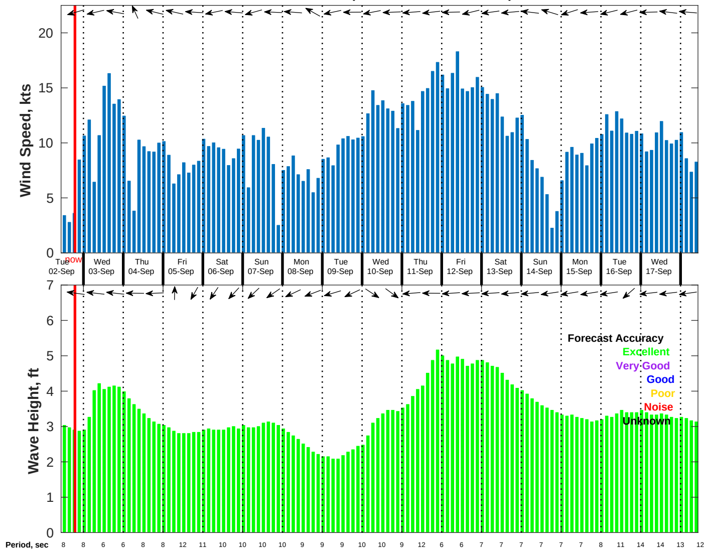
Wind & Wave Forecast for NDBC 52211 from 01-Sep-2025 11:00:00 to 17-Sep-2025 11:00:00
