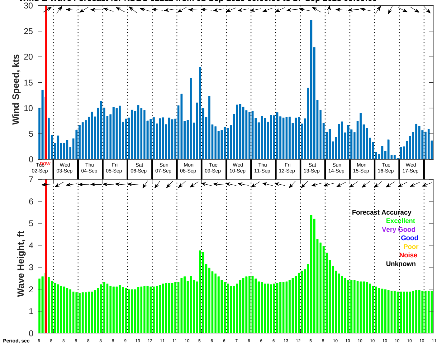
Wind & Wave Forecast for NDBC 52212 from 01-Sep-2025 09:00:00 to 17-Sep-2025 09:00:00
