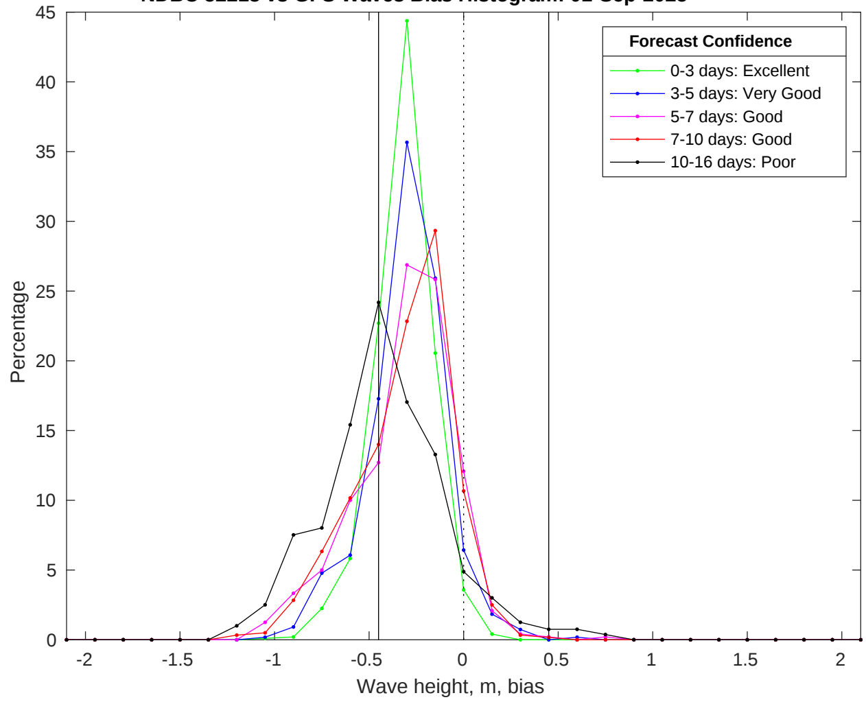
NDBC 52213 vs GFS Waves Bias Histogram: 01-Sep-2025
