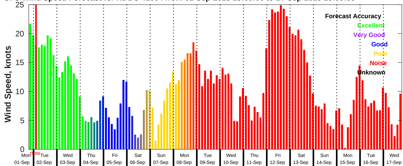
GFS Wind Speed Forecast for NDBC 41004 from 01-Sep-2025 19:00:00 to 17-Sep-2025 19:00:00
