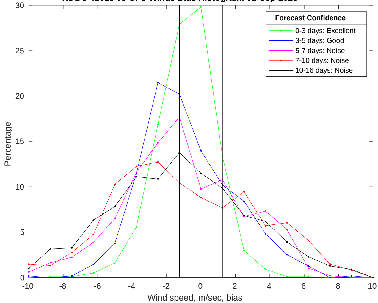
NDBC 41013 vs GFS Winds Bias Histogram: 02-Sep-2025
