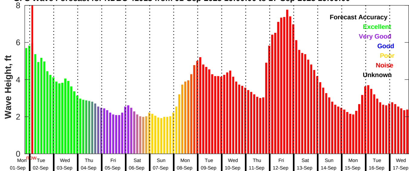
GFS Wave Forecast for NDBC 41013 from 01-Sep-2025 19:00:00 to 17-Sep-2025 19:00:00
