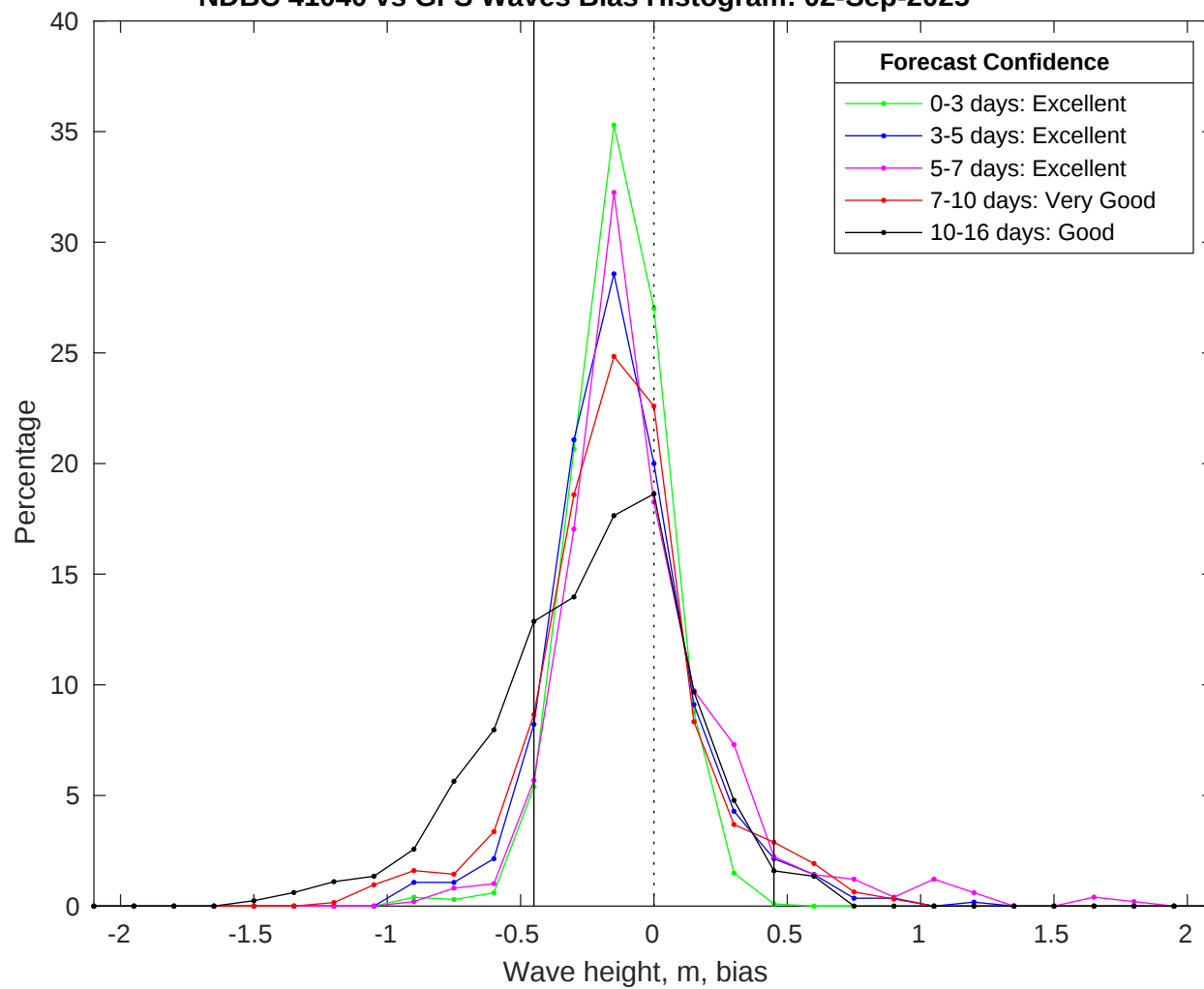
NDBC 41040 vs GFS Waves Bias Histogram: 02-Sep-2025
