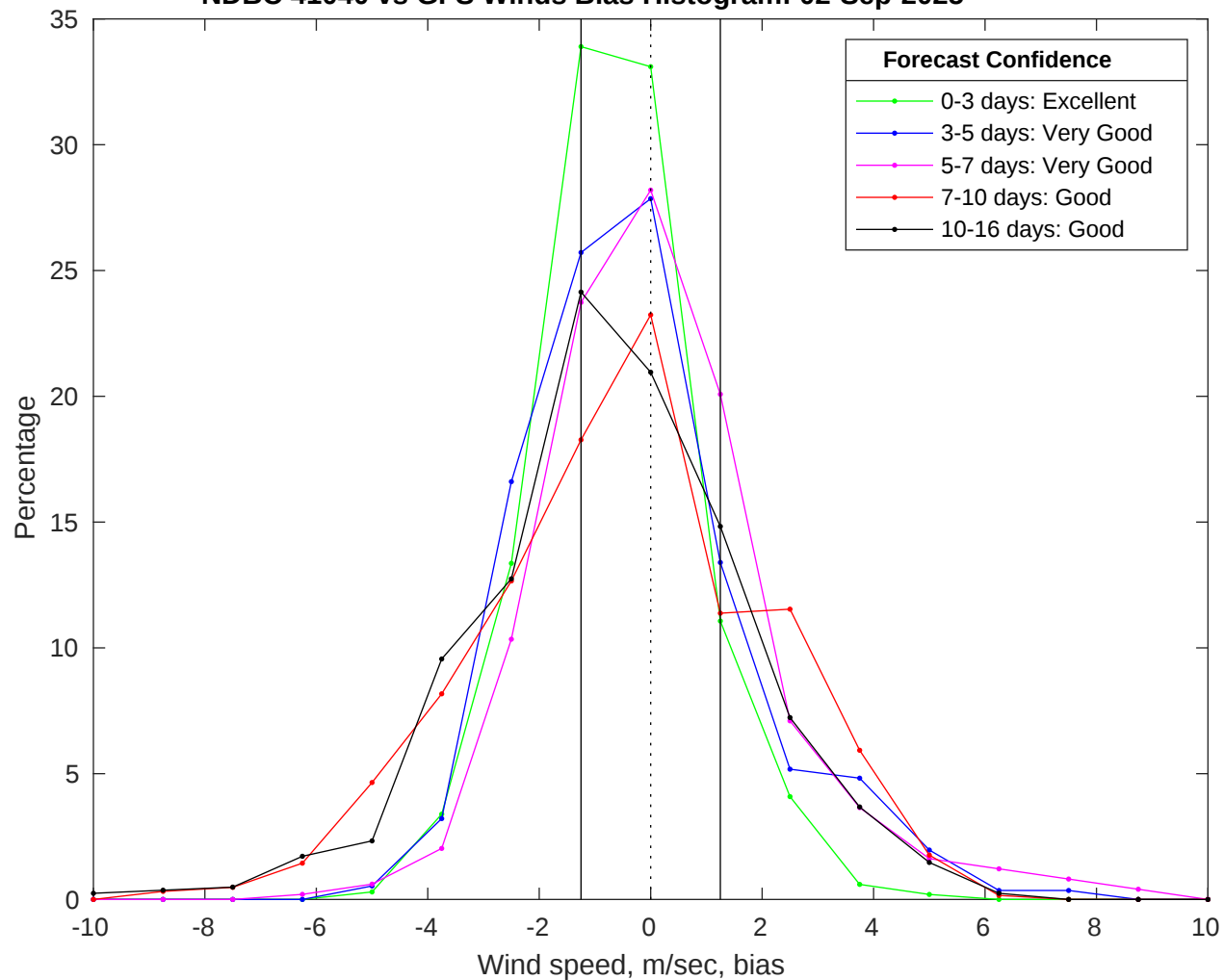
NDBC 41040 vs GFS Winds Bias Histogram: 02-Sep-2025
