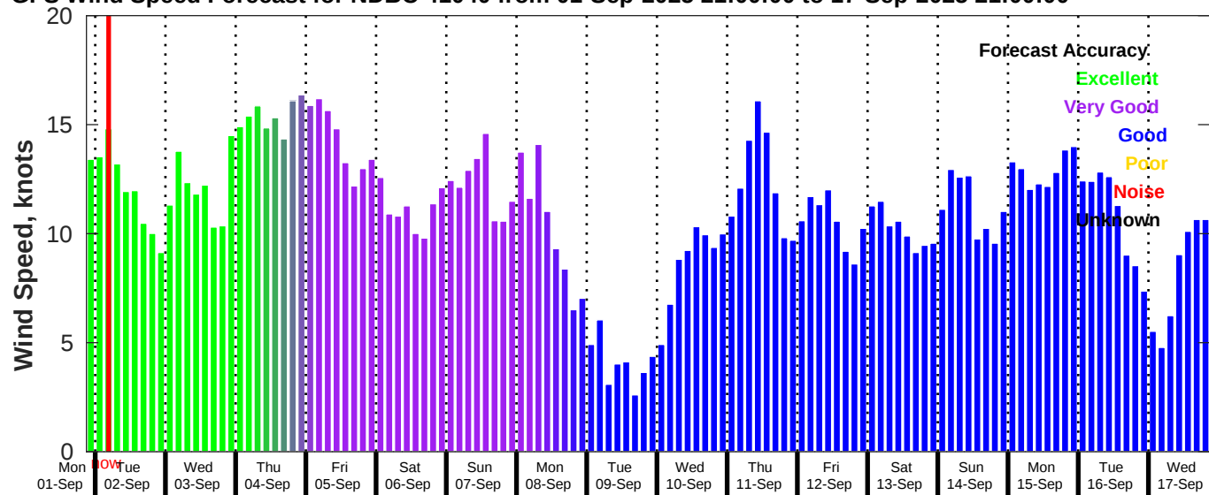
GFS Wind Speed Forecast for NDBC 41040 from 01-Sep-2025 21:00:00 to 17-Sep-2025 21:00:00
