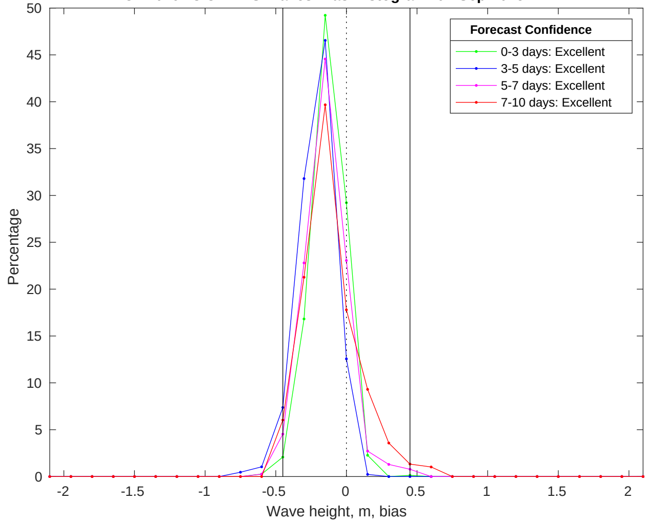
NDBC 42019 vs CMEMS Waves Bias Histogram: 02-Sep-2025
