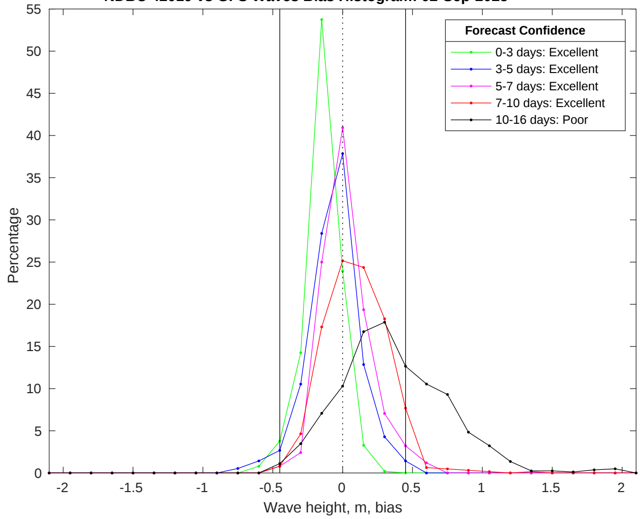
NDBC 42019 vs GFS Waves Bias Histogram: 02-Sep-2025
