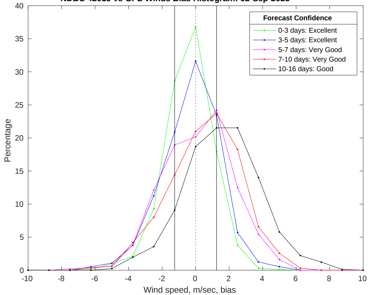
NDBC 42019 vs GFS Winds Bias Histogram: 02-Sep-2025
