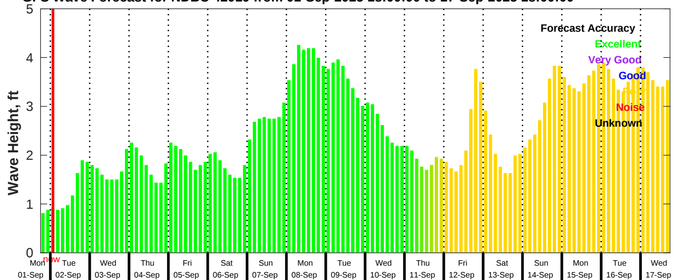
GFS Wave Forecast for NDBC 42019 from 01-Sep-2025 18:00:00 to 17-Sep-2025 18:00:00
