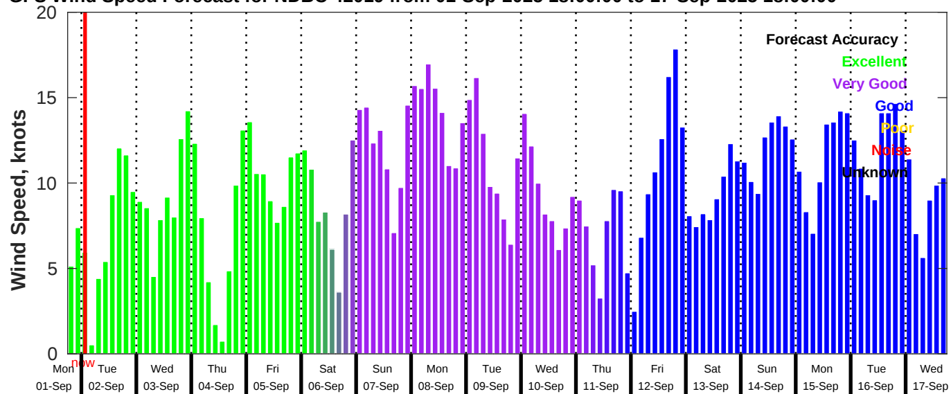
GFS Wind Speed Forecast for NDBC 42019 from 01-Sep-2025 18:00:00 to 17-Sep-2025 18:00:00
