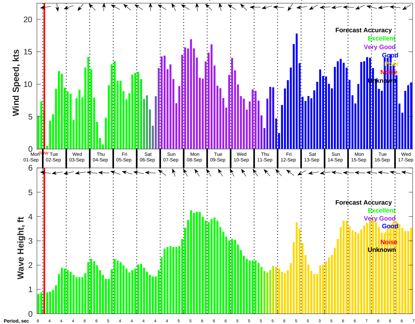
Wind & Wave Forecast for NDBC 42019 from 01-Sep-2025 18:00:00 to 17-Sep-2025 18:00:00
