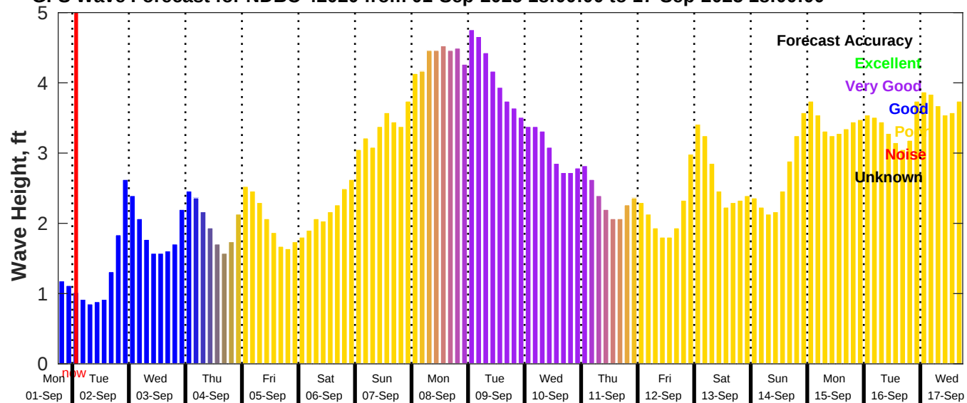
GFS Wave Forecast for NDBC 42020 from 01-Sep-2025 18:00:00 to 17-Sep-2025 18:00:00
