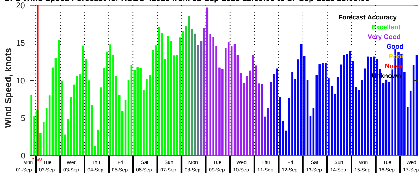
GFS Wind Speed Forecast for NDBC 42020 from 01-Sep-2025 18:00:00 to 17-Sep-2025 18:00:00
