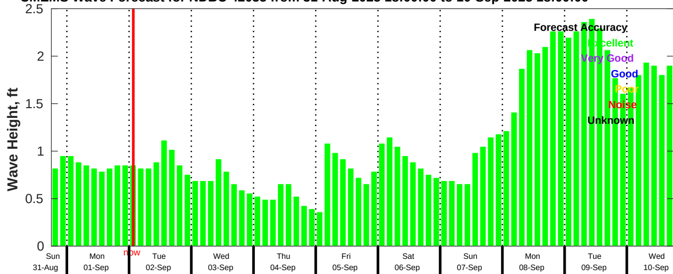
CMEMS Wave Forecast for NDBC 42035 from 31-Aug-2025 18:00:00 to 10-Sep-2025 18:00:00
