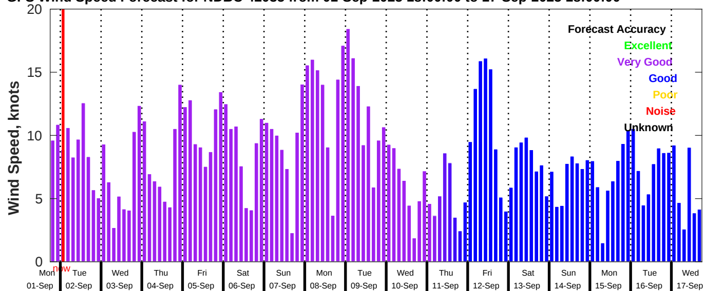
GFS Wind Speed Forecast for NDBC 42035 from 01-Sep-2025 18:00:00 to 17-Sep-2025 18:00:00
