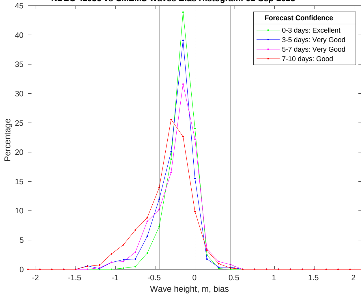
NDBC 42036 vs CMEMS Waves Bias Histogram: 02-Sep-2025
