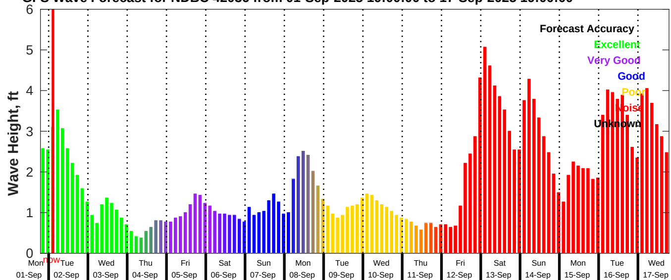
GFS Wave Forecast for NDBC 42036 from 01-Sep-2025 19:00:00 to 17-Sep-2025 19:00:00
