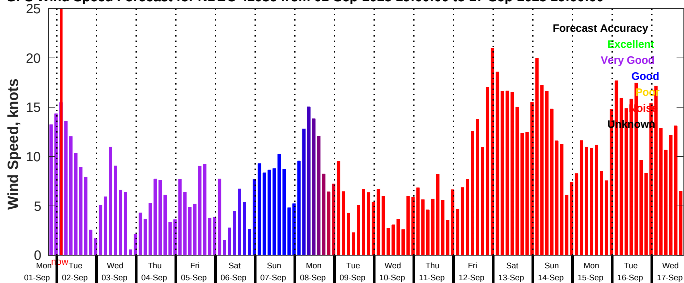
GFS Wind Speed Forecast for NDBC 42036 from 01-Sep-2025 19:00:00 to 17-Sep-2025 19:00:00
