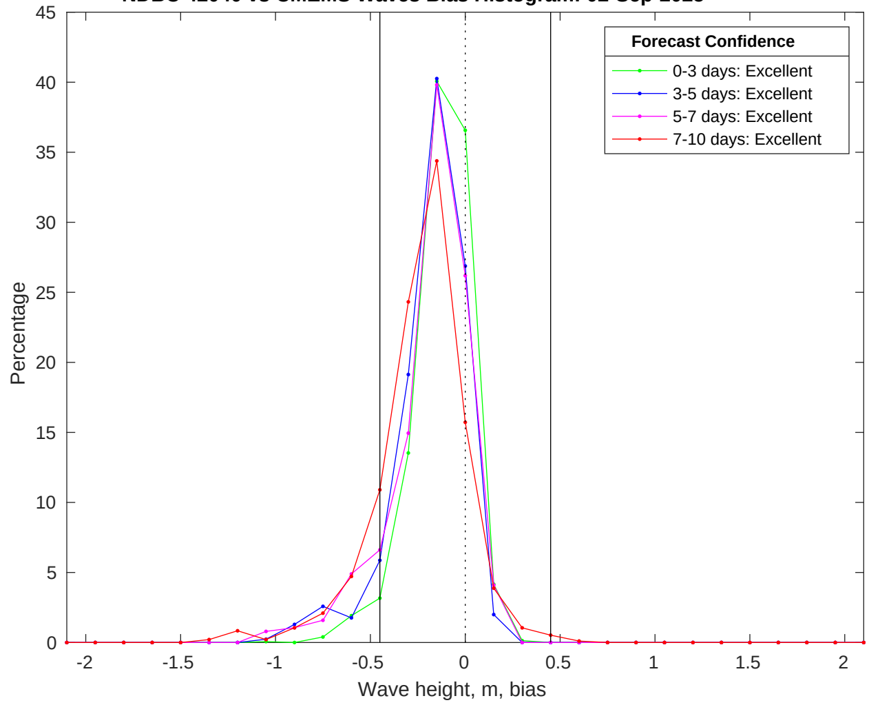
NDBC 42040 vs CMEMS Waves Bias Histogram: 02-Sep-2025
