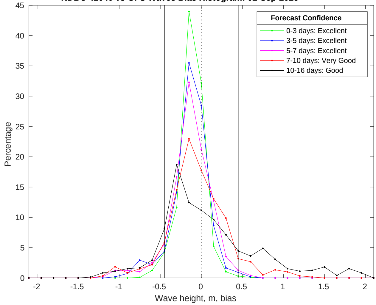
NDBC 42040 vs GFS Waves Bias Histogram: 02-Sep-2025
