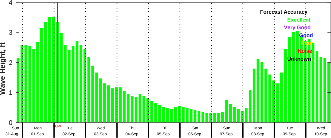
CMEMS Wave Forecast for NDBC 42040 from 31-Aug-2025 19:00:00 to 10-Sep-2025 19:00:00
