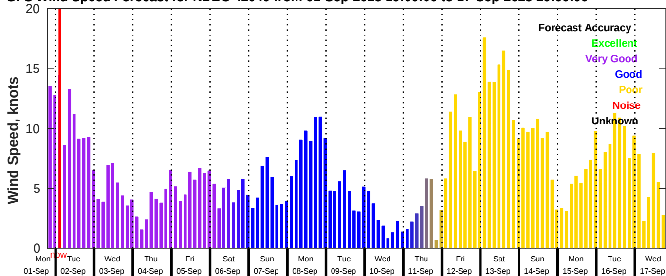
GFS Wind Speed Forecast for NDBC 42040 from 01-Sep-2025 19:00:00 to 17-Sep-2025 19:00:00
