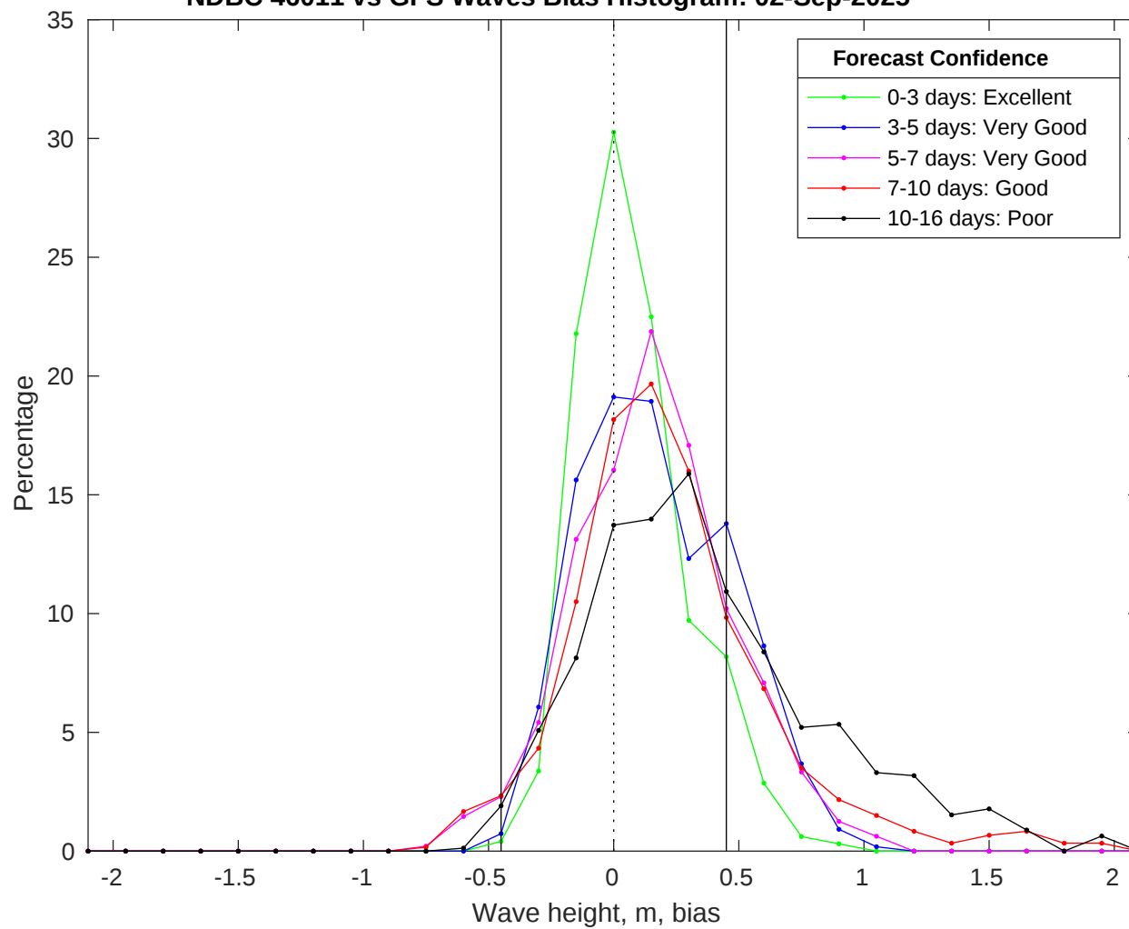
NDBC 46011 vs GFS Waves Bias Histogram: 02-Sep-2025
