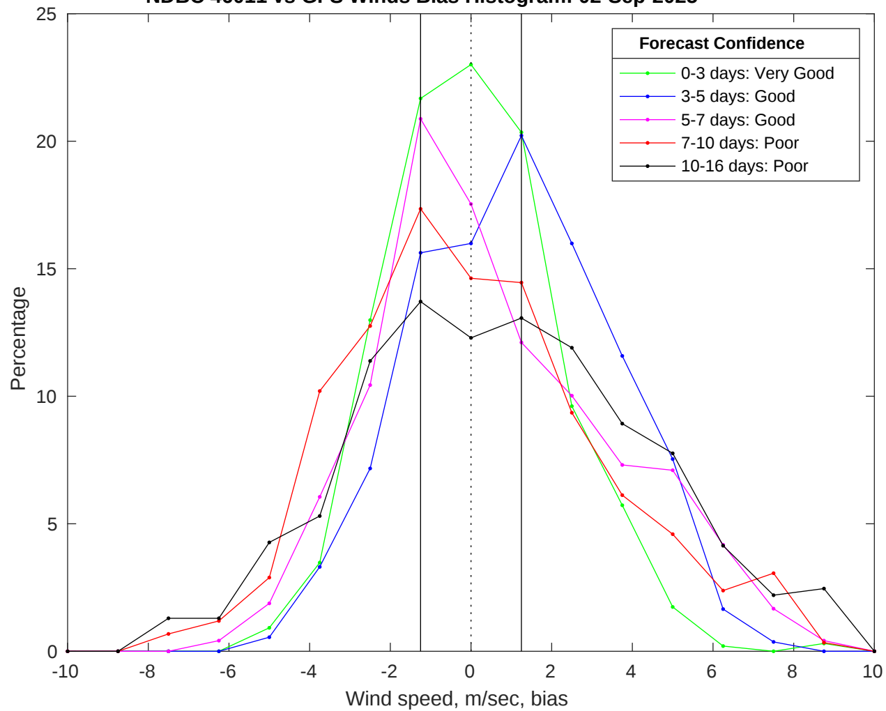
NDBC 46011 vs GFS Winds Bias Histogram: 02-Sep-2025
