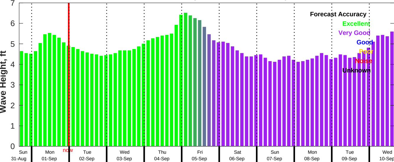
CMEMS Wave Forecast for NDBC 46011 from 31-Aug-2025 16:00:00 to 10-Sep-2025 16:00:00
