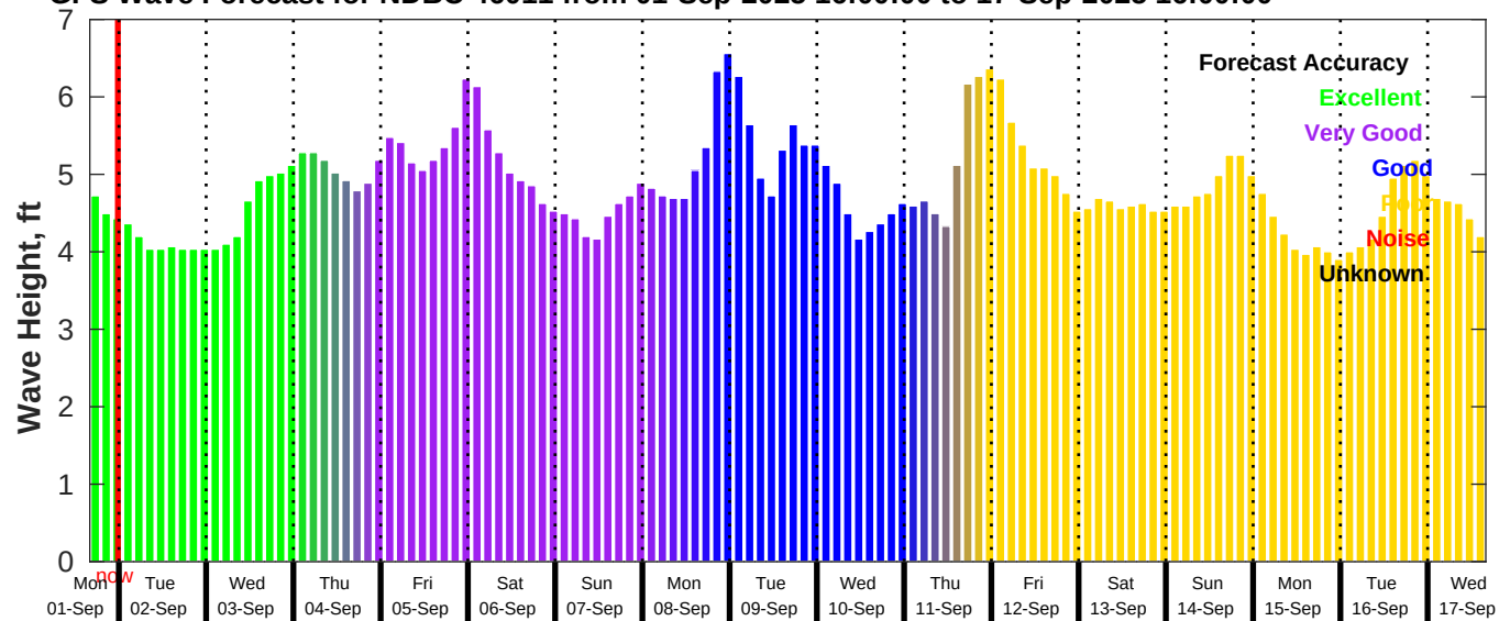
GFS Wave Forecast for NDBC 46011 from 01-Sep-2025 16:00:00 to 17-Sep-2025 16:00:00
