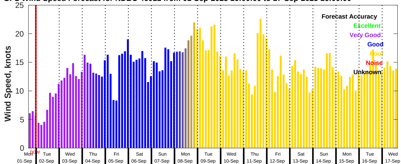
GFS Wind Speed Forecast for NDBC 46011 from 01-Sep-2025 16:00:00 to 17-Sep-2025 16:00:00
