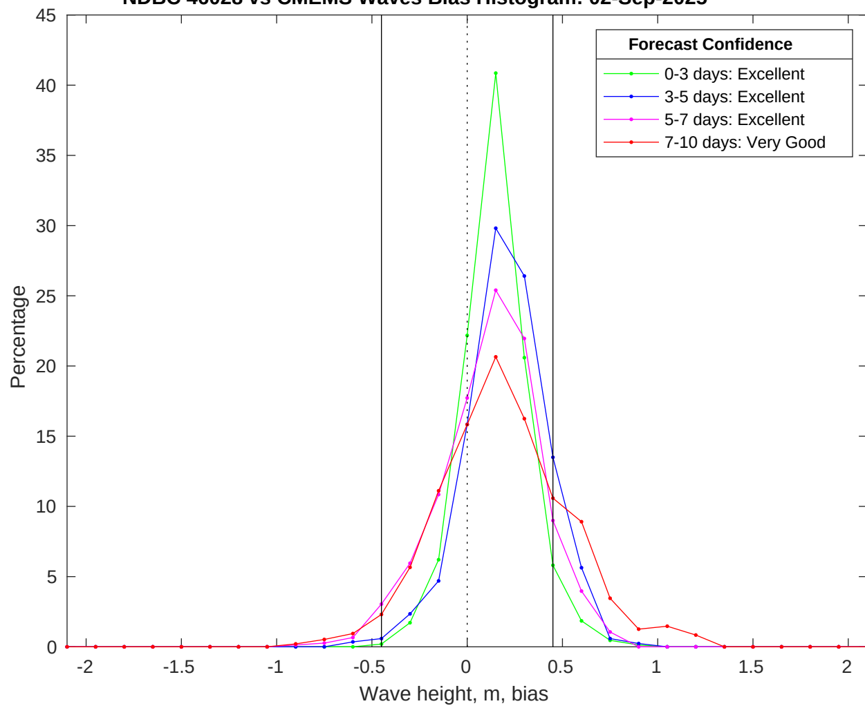
NDBC 46028 vs CMEMS Waves Bias Histogram: 02-Sep-2025
