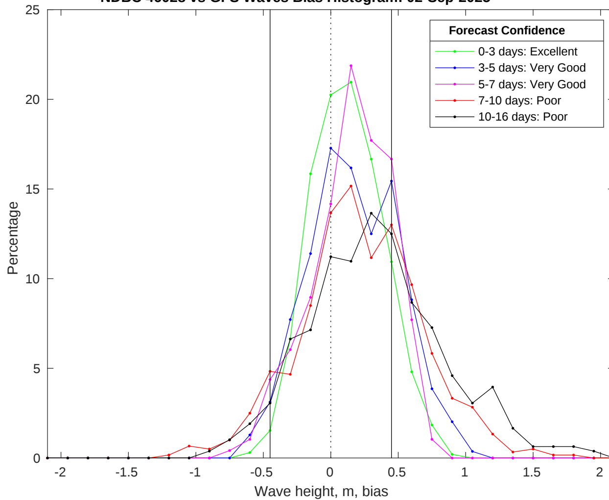
NDBC 46028 vs GFS Waves Bias Histogram: 02-Sep-2025
